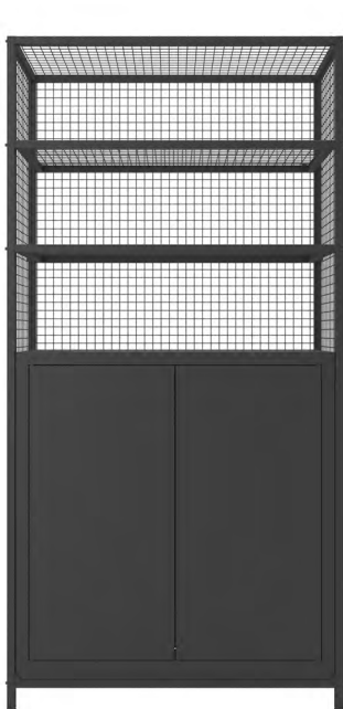
LOV 6C CODE: LOV 0306030304 H. x W. x D. : 2080 x 1053 x 445 [mm] SBM 102M Double door cabinet 2 shelves inside
