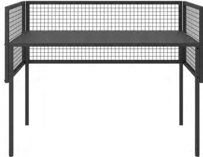
Lov 9 CODE: LOV 0609000006 H. x W. x D. : 752 x 1307 x 620 Desk with a 1.5 mm thick steel top, with adjustable extension.
